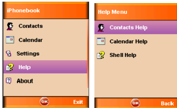
Figure 17: Help Options
