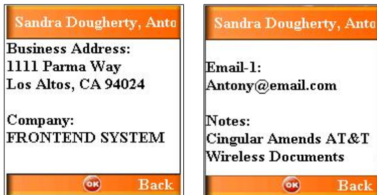
Figure 9: Details display
