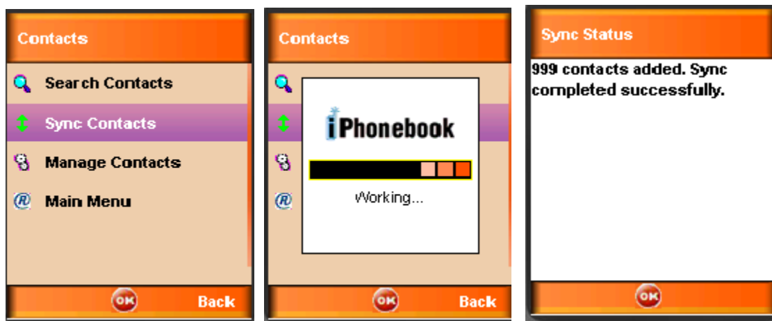
Figure 12: Sync Contacts option
