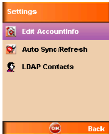
Figure 13: Settings option
