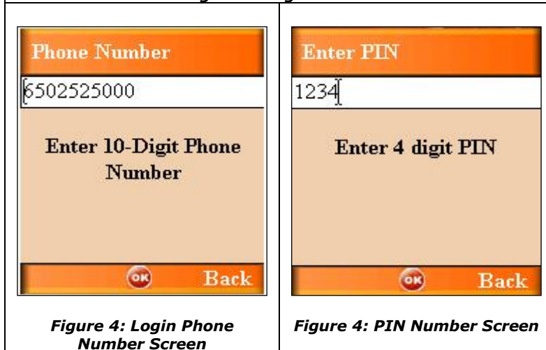
Figure 4: Login Screen
