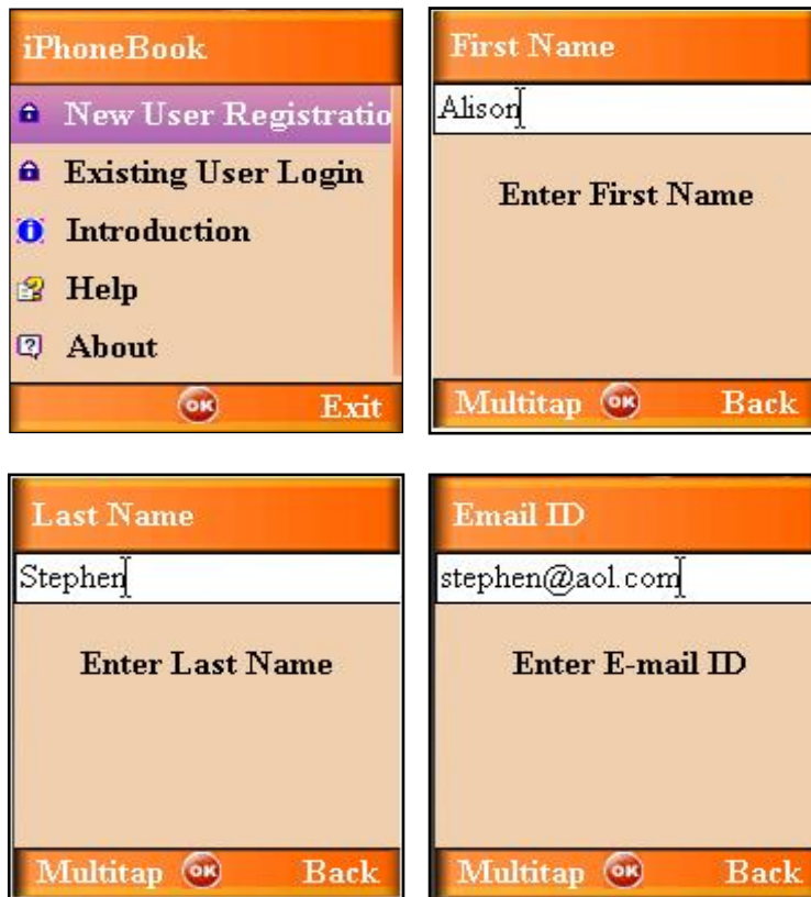
Figure 3: Registration Options
