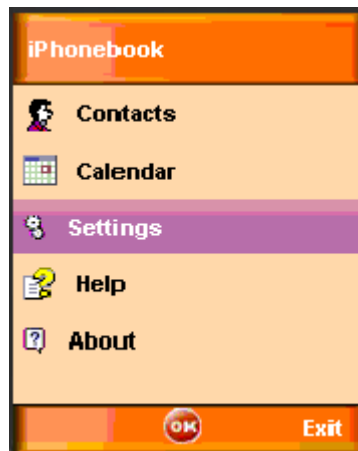
Figure 13: Settings option
